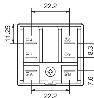
62.32-0300
