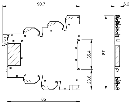
Tipi 39.70 39.71 Terminali Push-in
