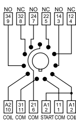
90.03
