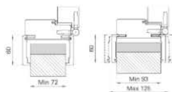
TP/L6 72 MM - 100 MM
