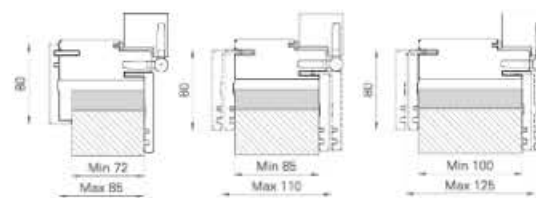
TLS-A/L8 72 MM - 85 MM - 105 MM
